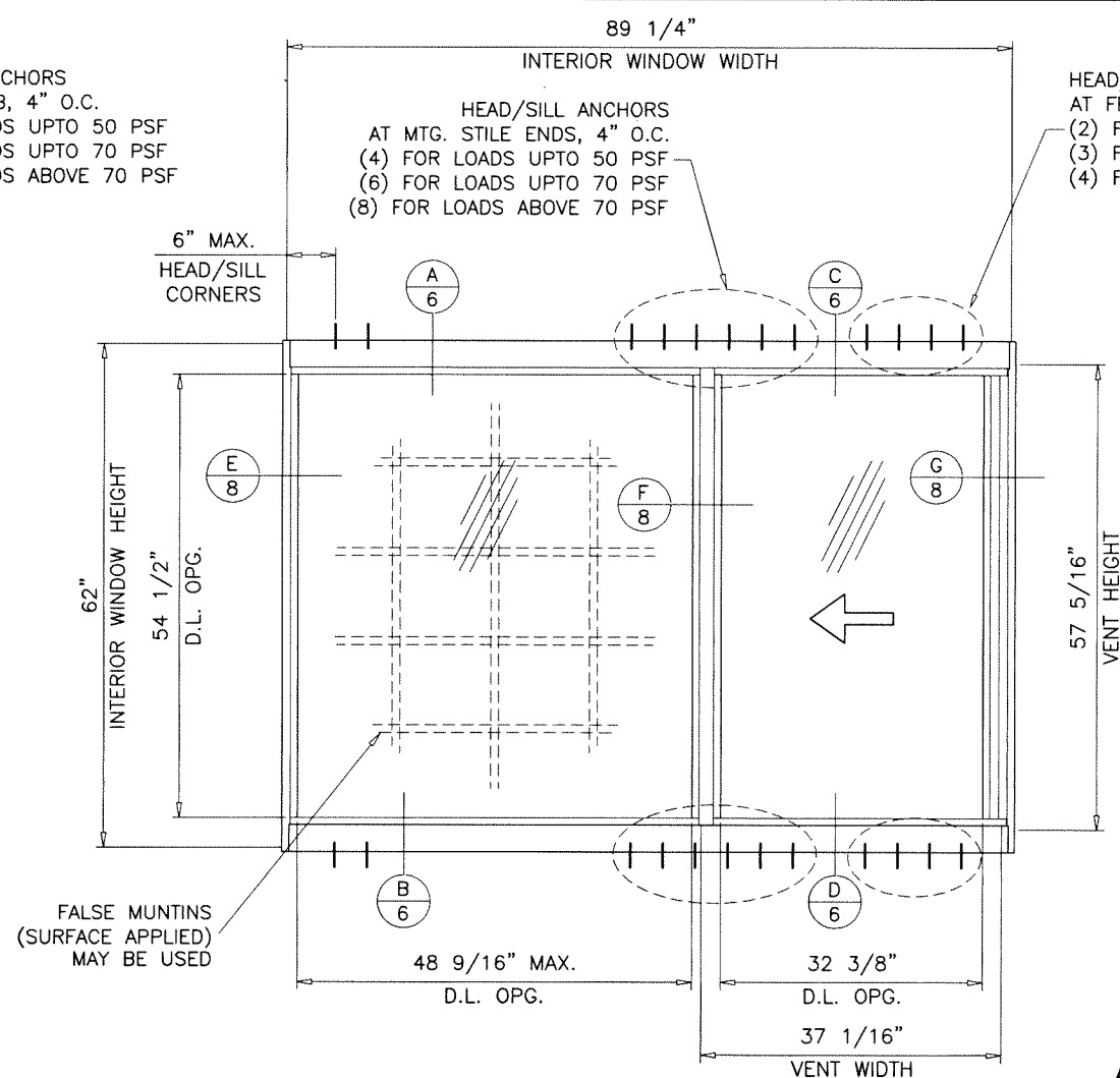
TYPICAL ELEVATIONS
