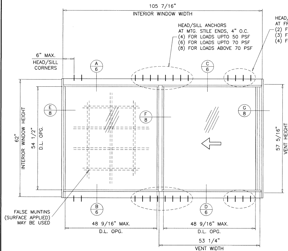
TYPICAL ELEVATIONS
