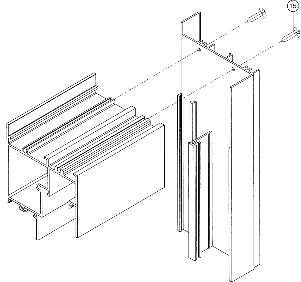
FRAME TOP/BOTTOM CORNER
